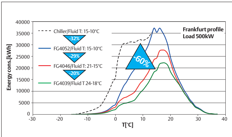
Liebert HPC-M with SmartAisle™ compared with a conventional chiller installation.
